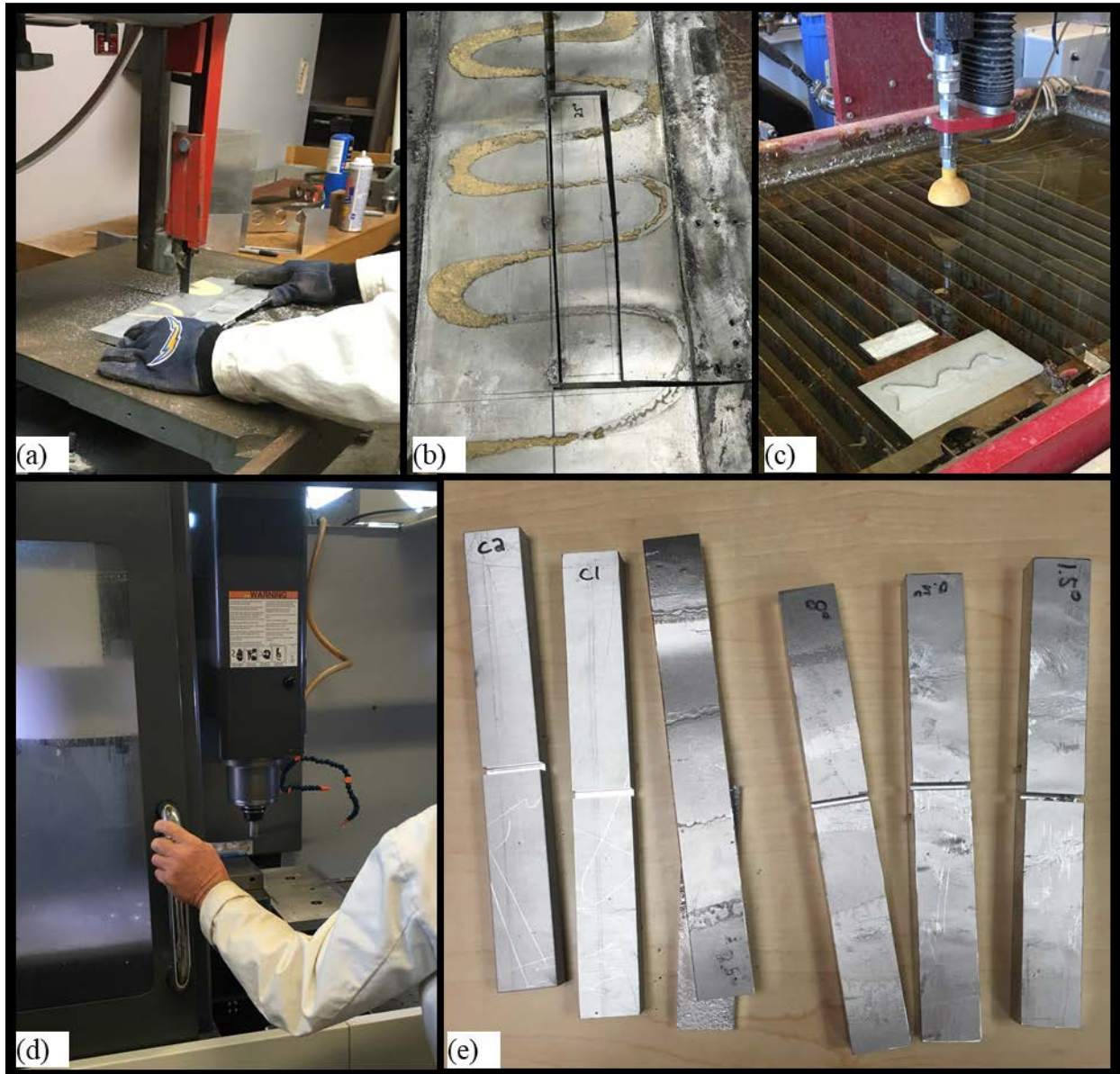
Figure 4-8: Fabrication of tensile shear specimens. (a) & (b) Band saw cuts to rough dimensions out of weld specimens. (c) Water jet cuts from control plate. (d) CNC milling to final dimensions. (e) Final specimens, showing one of the 2.5° specimens that failed during fabrication.
