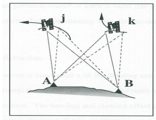
Figure 5: Triple Differencing
