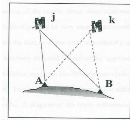
Figure 4: Double Differencing (Adapted from RSMS Lecture “GPS Phase and Range Equations, 26 June 2001)
