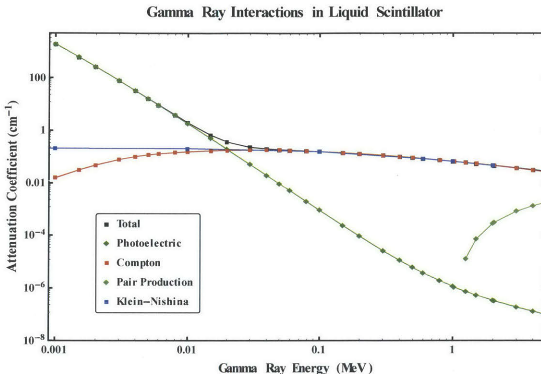
Figure 2.13. Attenuation coefficients in organic liquid scintillator for 1 keV to 5 MeV gamma rays. 29 Compton scatter is the primary interaction for gamma ray energies between 0.1 MeV and 1.0 MeV. Klein-Nishina calculation shown for comparison.
