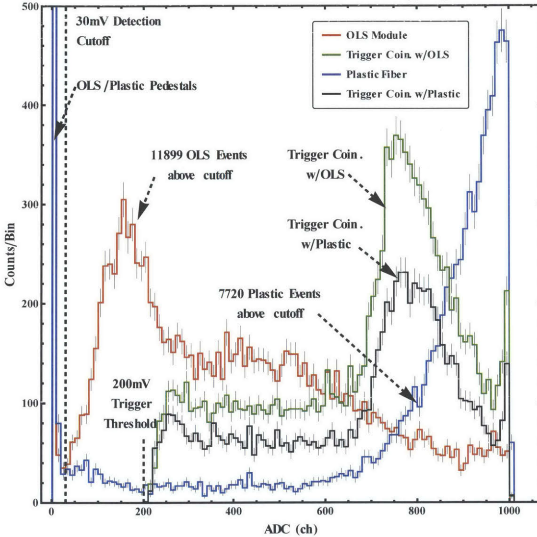
Figure 5.2. Comparison of OLS module and plastic fiber pulse height spectra. The OLS module and plastic fiber signals were collected when a large rectangular scintillator (trigger) measured an event above ~200 mV. Of the 140,000 triggered events, less than 20,000 were coincident with OLS module or plastic fiber signals over 30 mV.
