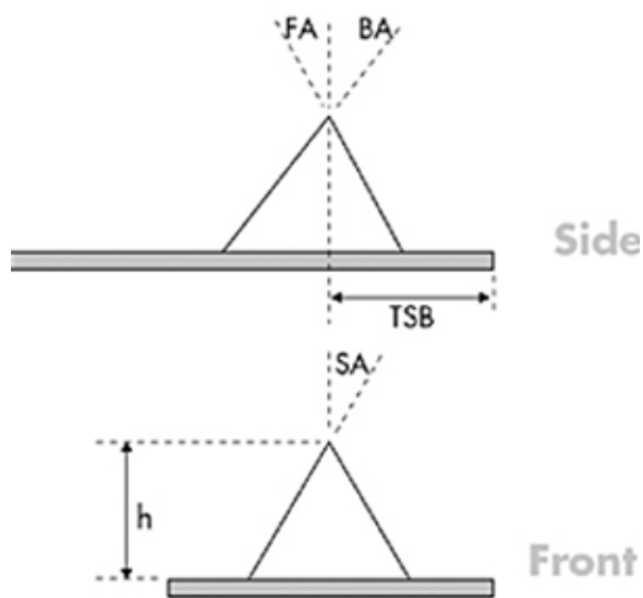
Figure 13. Bruker AFM Probe Geometry Specification [14]. Reprinted with permission from Bruker Corporation. TSB is the tip setback distance, the distance from the end of the cantilever to the vertical axis of the tip. FA, BA, SA, and h are as defined in Table 1.
