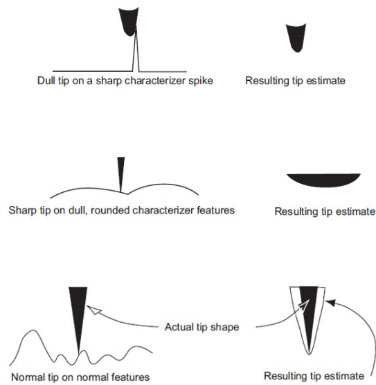
Figure 12. Tip Estimates Given by Different Surface Features [16]. Reproduced with permission from Bruker Corporation.
